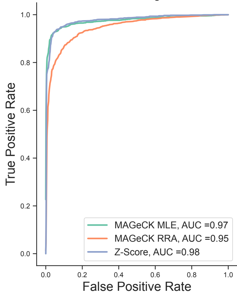
Brunello A375 screen gene-level ROC
