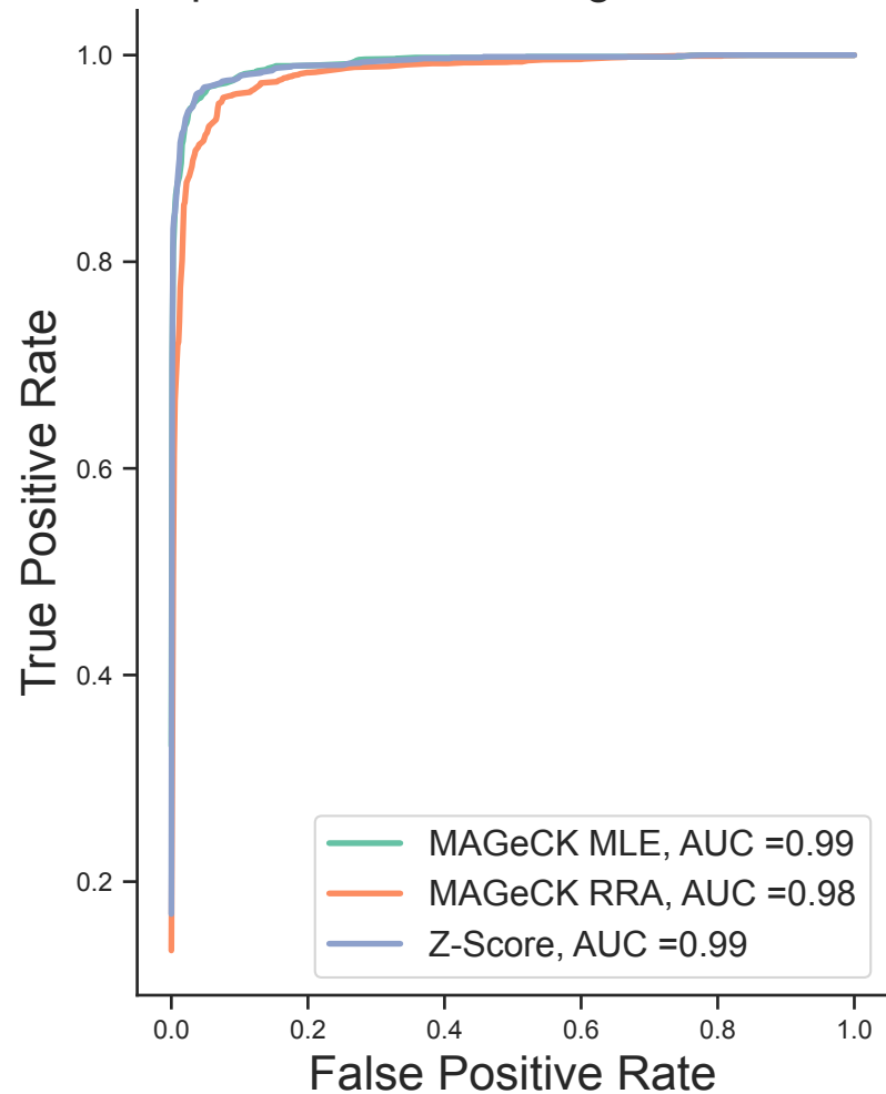
Jacquere A375 screen gene-level ROC
